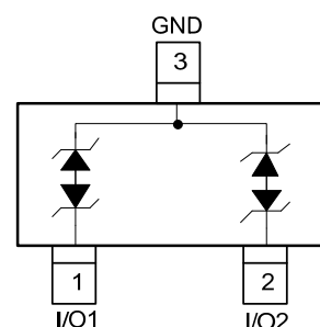
Circuit diagram
